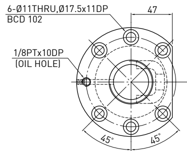
D-D VIEW
